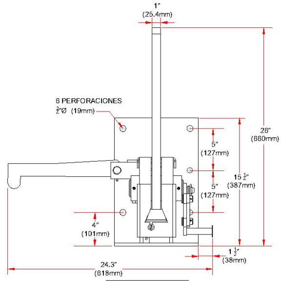
Vista Frontal
